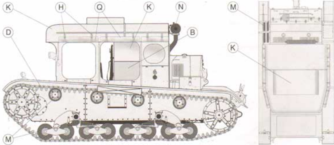
Ciężnik artyleryjski C7P Nr 8391 z 1 PAN w jednobarwnym malowaniu. Heavy artillery tractor C7P No 8391 from 1st Heaviest Artillery Regiment in green overall paint.
